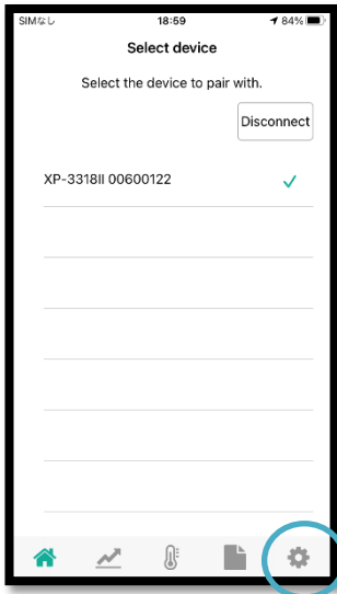
Settings button
